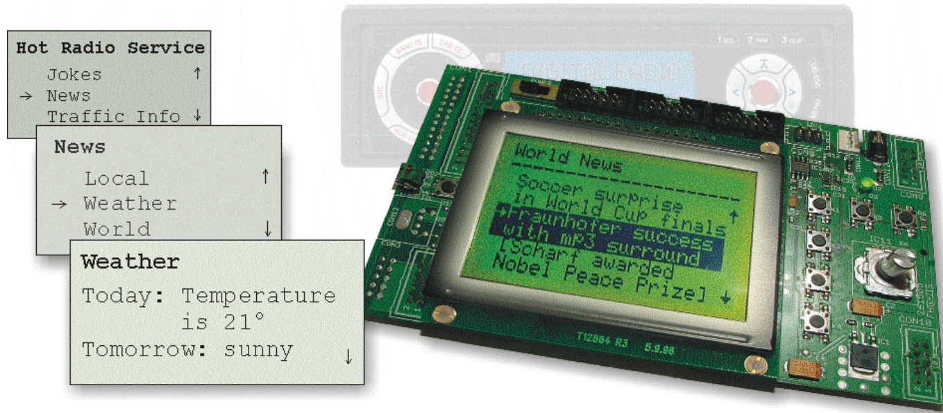
Embedded Journaline decoder for integration in microcontrollers
